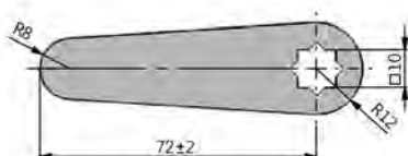
S1C7200 標配擋片 standard Cam
