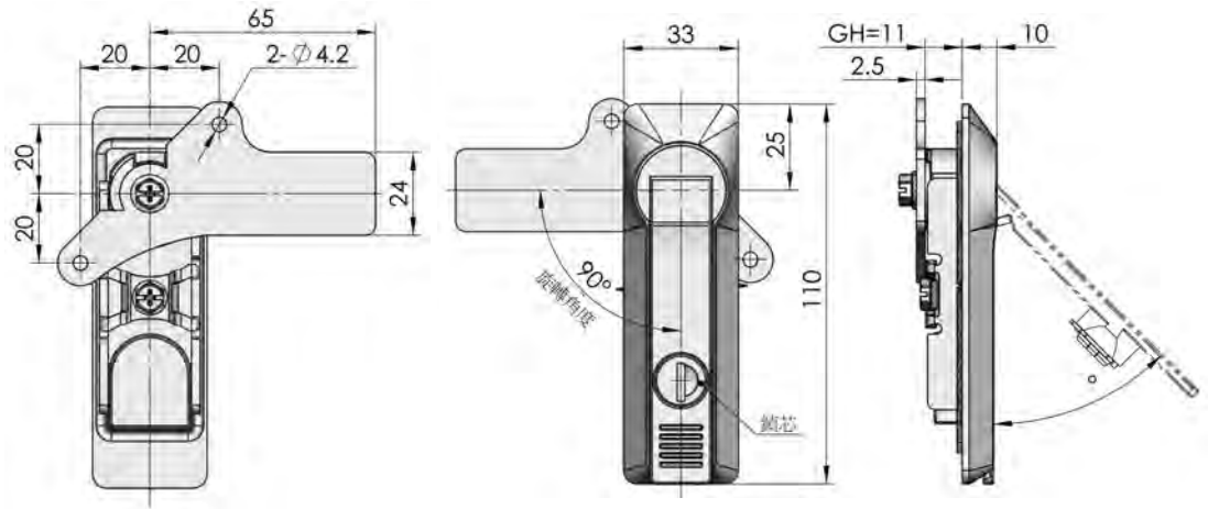
MS-723-2 (附鎖芯 Locking)
