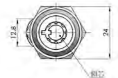
鎖芯
