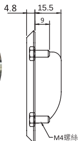
螺柱型(適用板厚:6mm內) Outside Stationary type HP-008-1
