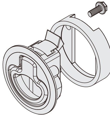
安裝螺絲 M5X12 (Supplied)
